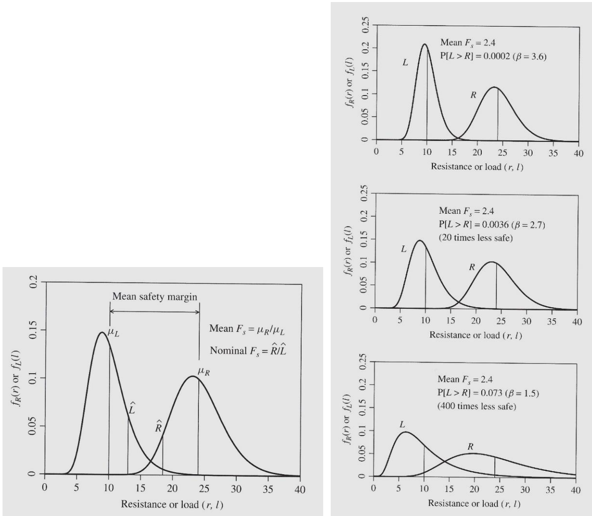
Fig. 3.4: Distribution functions for load and resistance defining the safety margin. Left: general representation, Right: influence of scattering on safety in case of identical mean values (Fenton & Griffiths, 2008).
