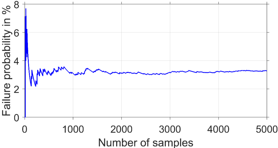
Fig. 5.6.3: Failure probability calculated by the Monte Carlo simulation
