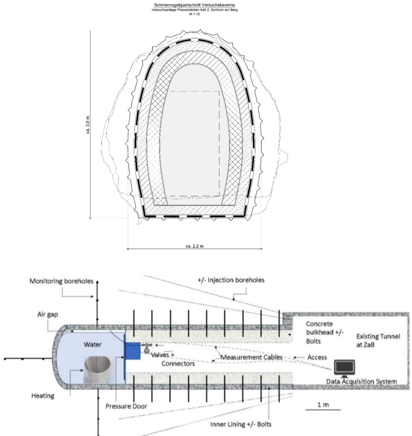
Fig. 3.5: Preliminary layout of HEATROCK project (Villeneuve, 2025)
