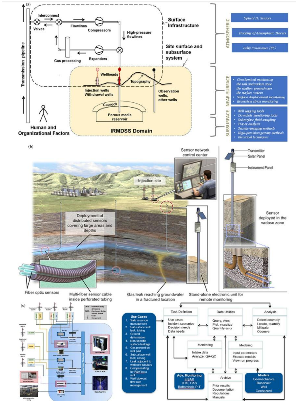
Fig. 12.2: Risk monitoring for underground hydrogen storage (Lin et al. 2026)
