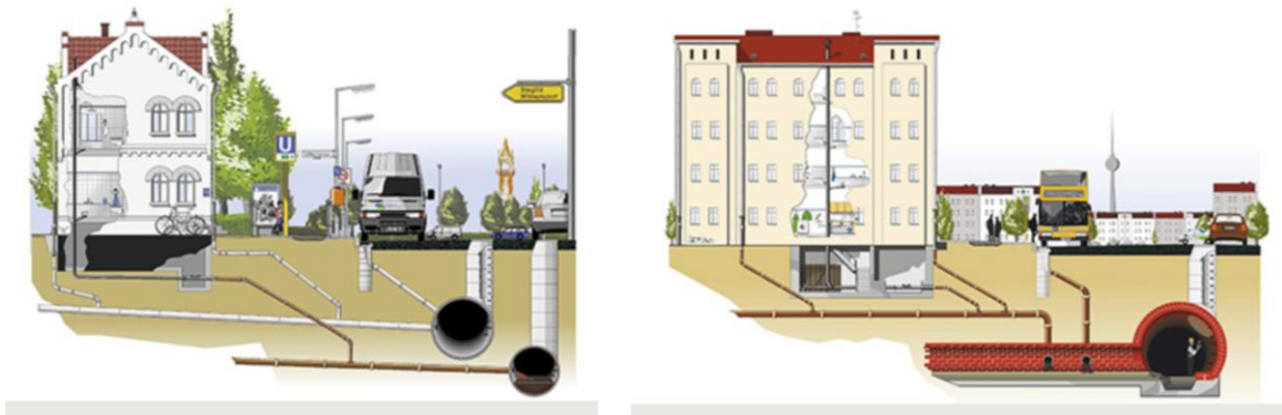
Fig. 6.1: Illustration of waste water systems in a city (BW, 2020)
