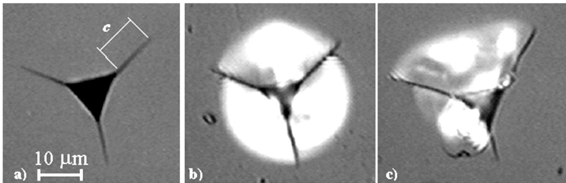
Fig. 3.16.5: Optical micrographs of cube-corner indentations (Volinsky et al., 2003)
