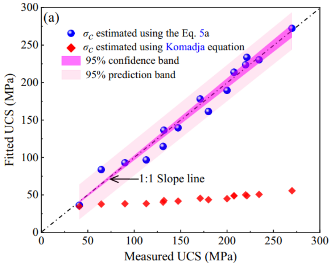
Fig. 3.16.13: UCS for different types of rock deduced from nanoindentation tests using different methods compared to macroscopic measured values (Liu et al., 2024)
