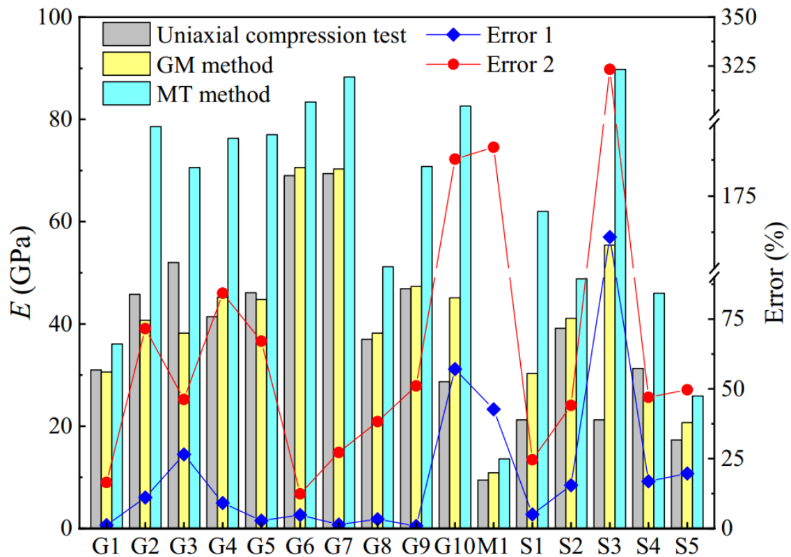
Fig. 3.16.12: Young's modulus for different types of rock deduced from nanoindentation tests using different methods compared to macroscopic measured values (Liu et al., 2024)
