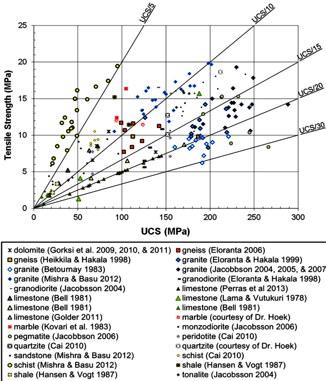
Fig. 3.10.4: Relation between UCS and tensile strength (Perras & Diederichs, 2014)
