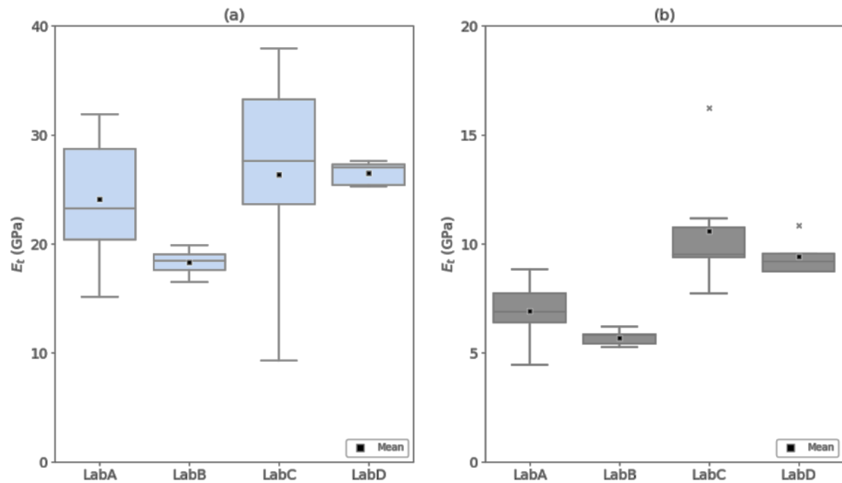
Fig. 3.8.5: Boxplot for Young's moduls obtained by 4 different labs using direct tension tests, (a) Blaco Mera granite, (b) Cotta sandstone
