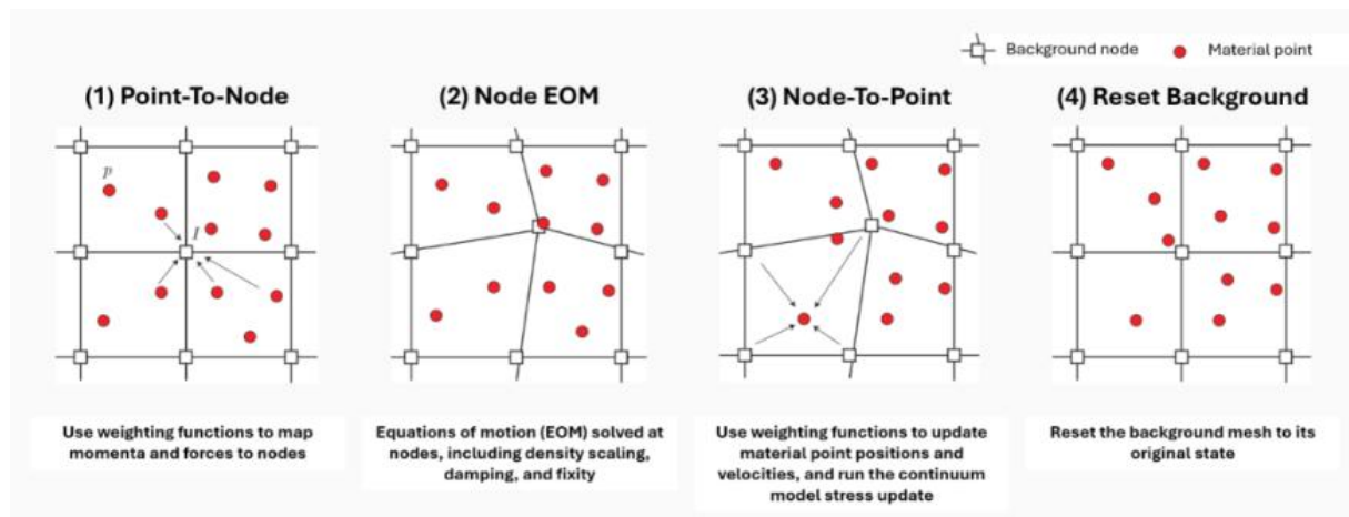
Abb. 5.6.2: MPoint's solution cycle consists of four primary operations between Lagrangian material points (P) and a stationary Eulerian background grid (Itasca, 2026)
