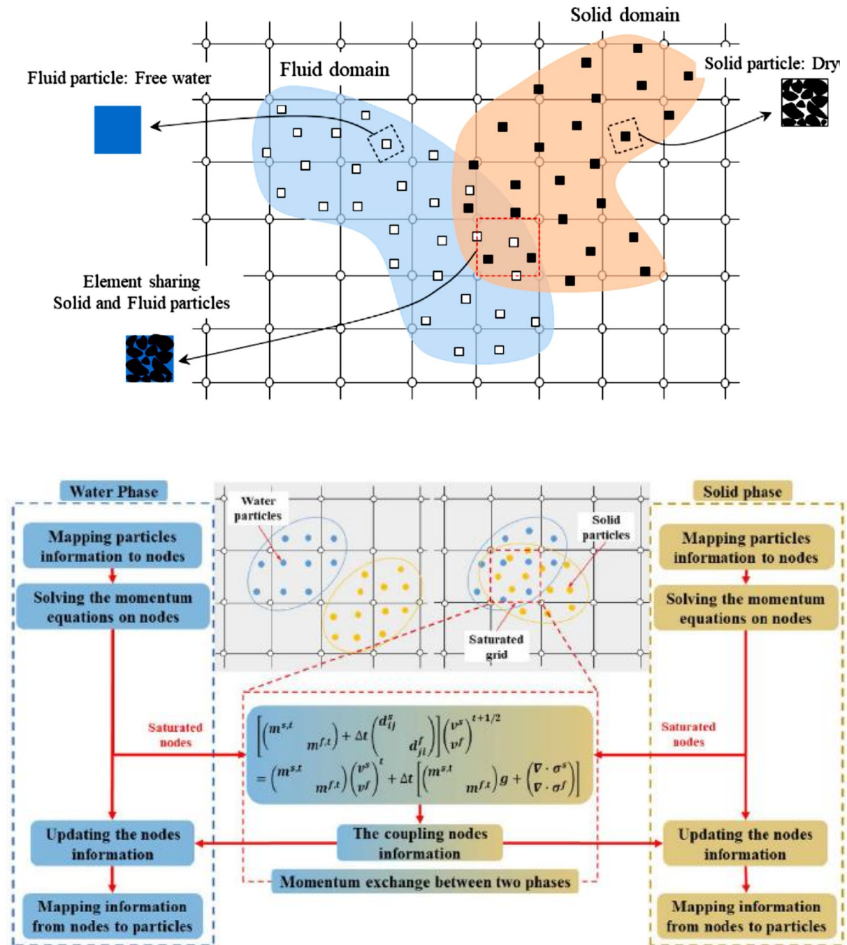
Fig. 5.6.3: HM-coupled MPM for simulation of a landslide problem (Du et al., 2022)
