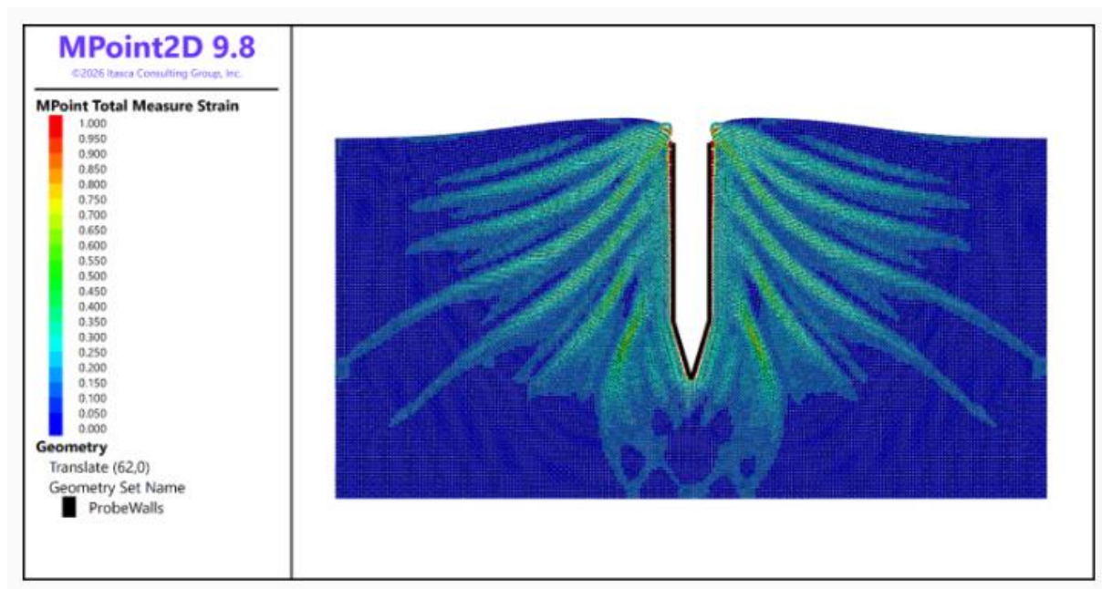
Fig. 5.6.4: Penetration of a probe into the ground; Total strain contours (Itasca, 2026)
