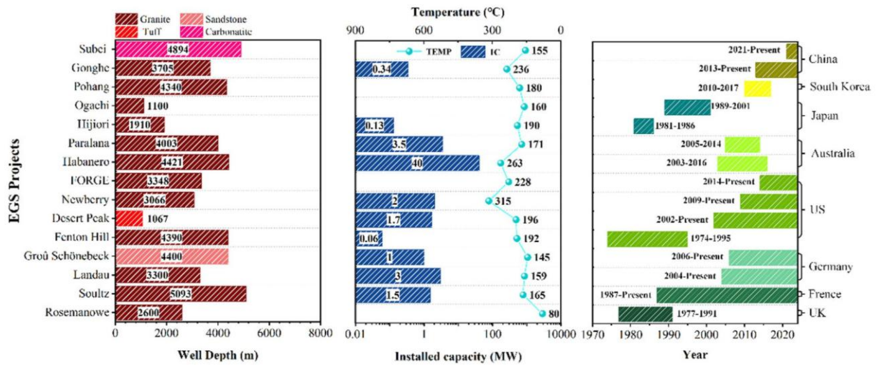
Fig. 1.6: Status of major global EGS projects (Li et al., 2025)
