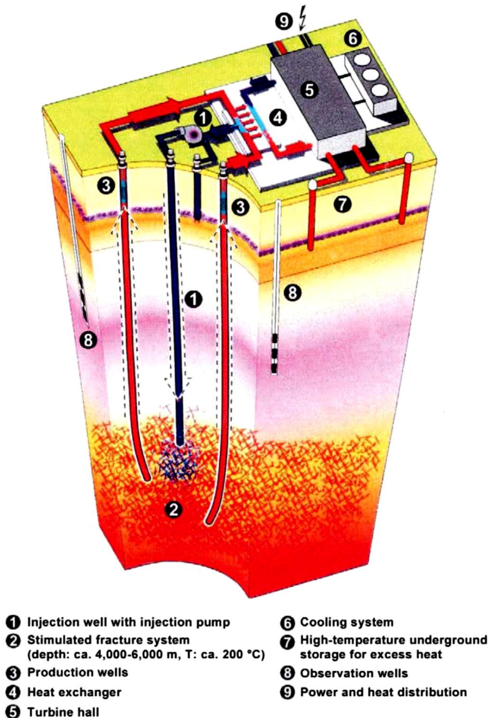
Fig. 3.1: Basic structure of a HDR system with its main components (LIAG, 2017)
